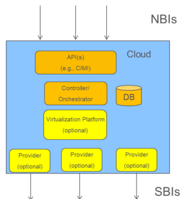
342 343 Figure 11 – Proposed Cloud Provider architecture
