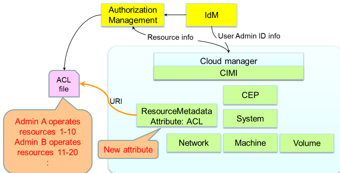
296 297 Figure 6 – Authorization metadata management example
